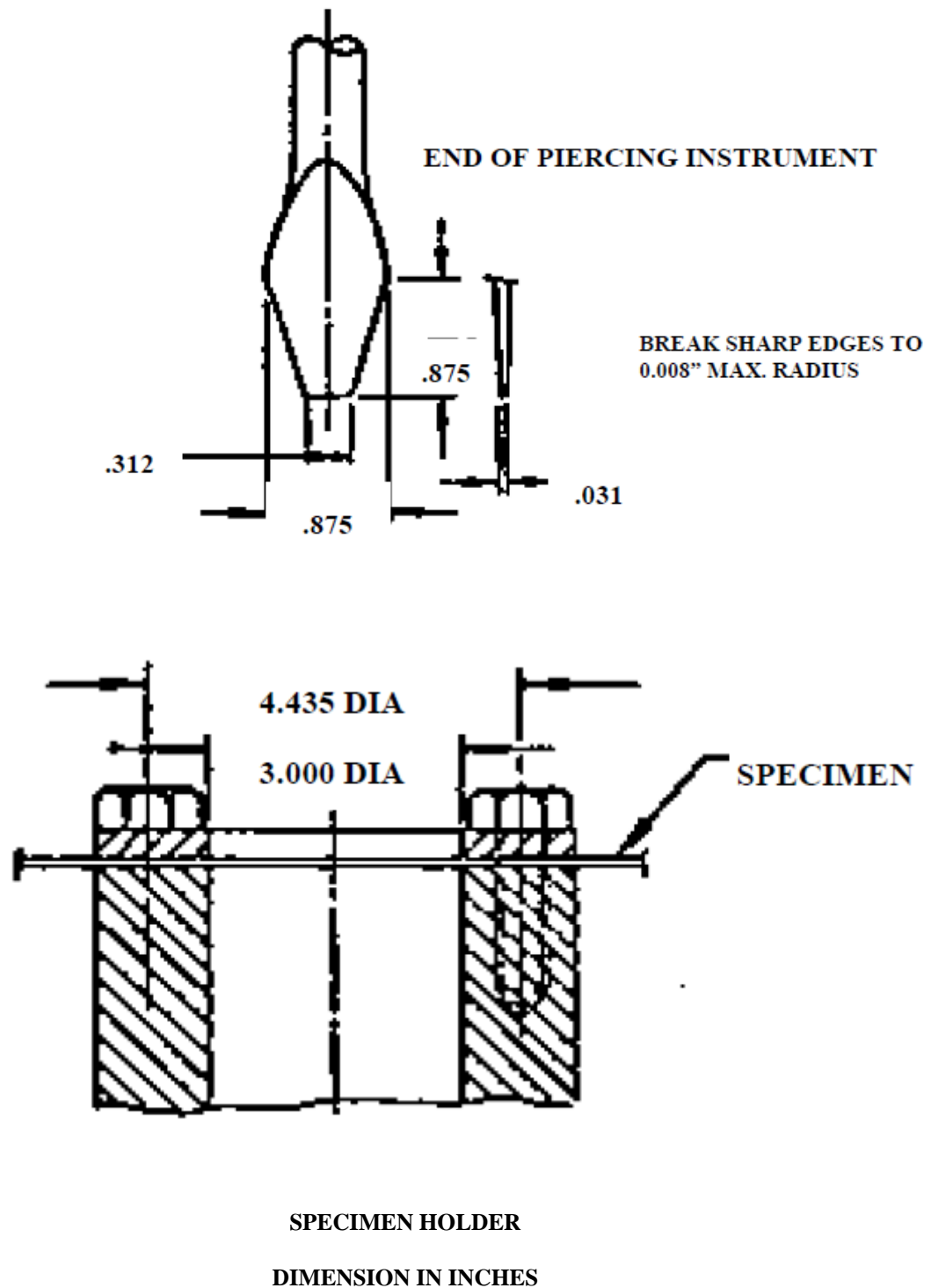
FIGURE 1. PIERCING INSTRUMENT AND SPECIMEN HOLDER
